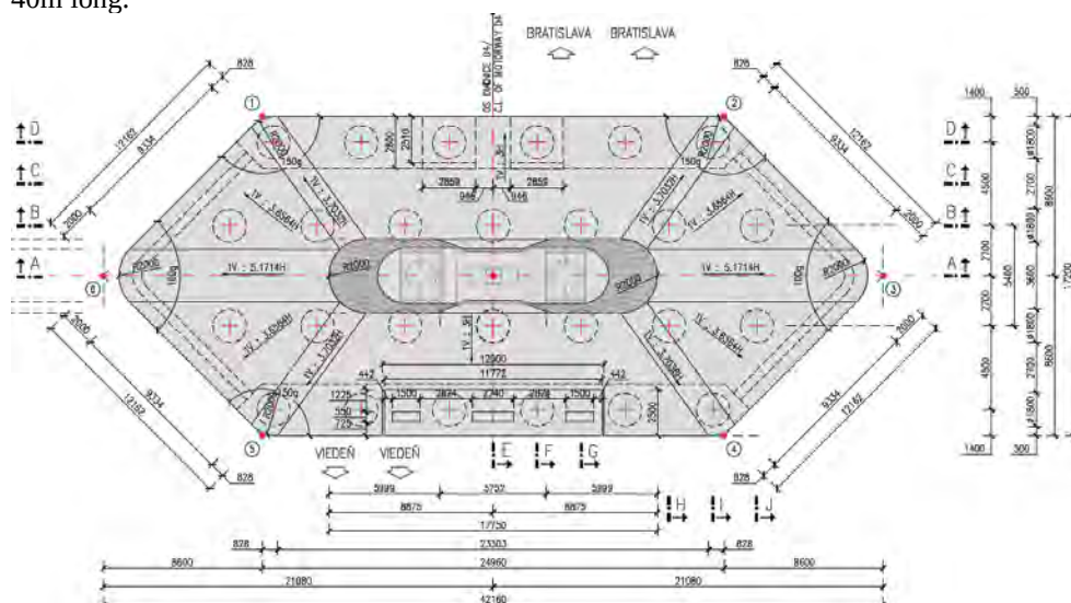
Plan view of a principal pier, based on an hydrodynamic hexagonal pile cap supported by 26Ø1.8m piles.
