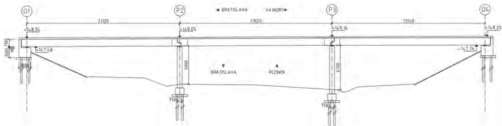
Figure 1 Scheme of the bridge - longitudinal section
