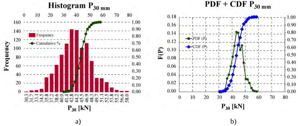
Obr. 6 – a) Histogram predpínacej sily pre \Delta\sigma_{c,30} ;
