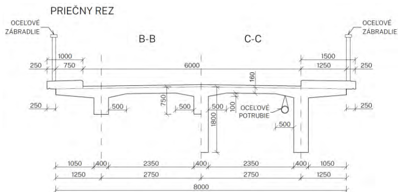
Obr. 2 – Priechy rez v poli (B-B) a nad vzperou (C-C).
